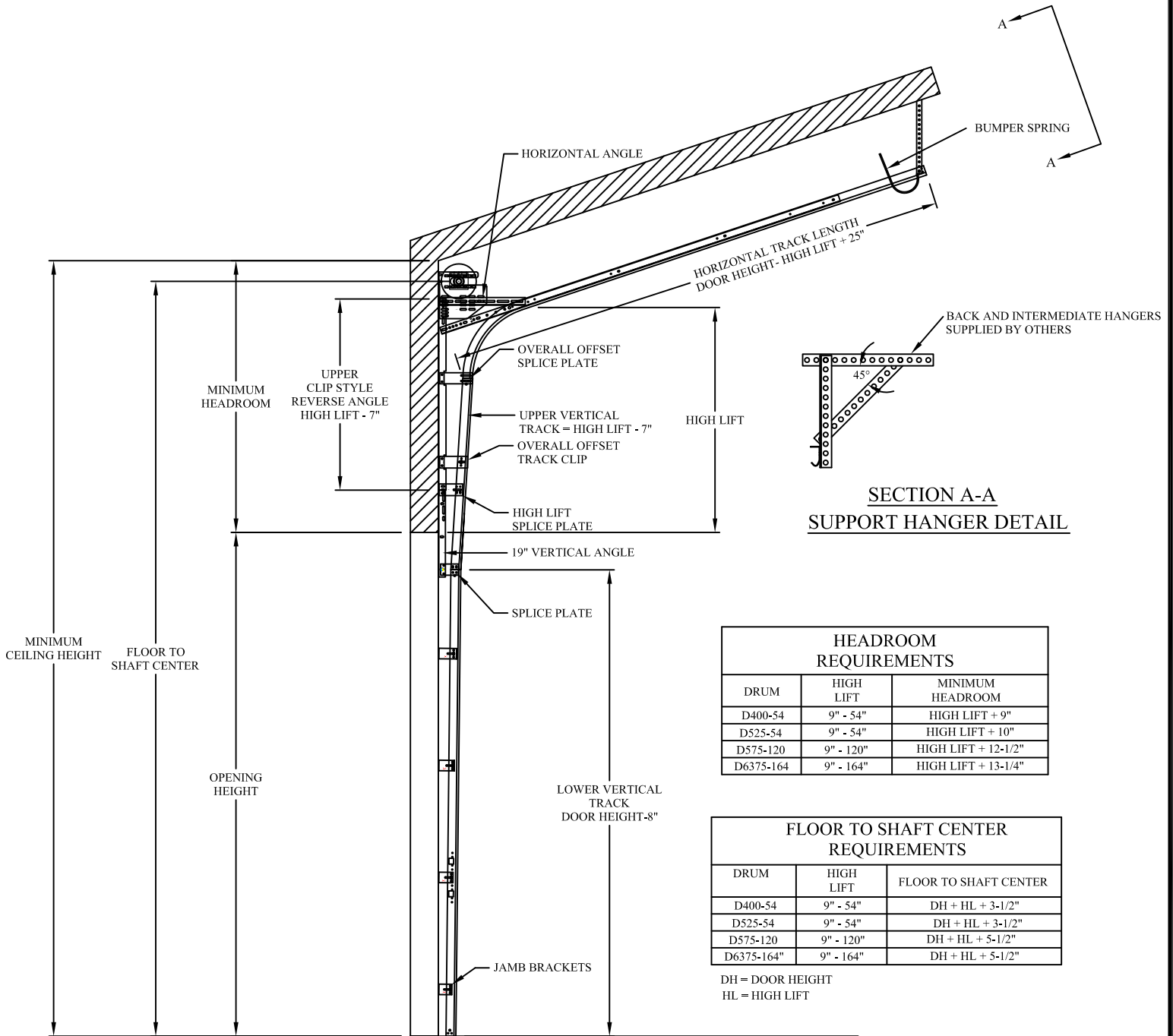
HIGH LIFT BRACKET MOUNT TRACK SET DETAIL
