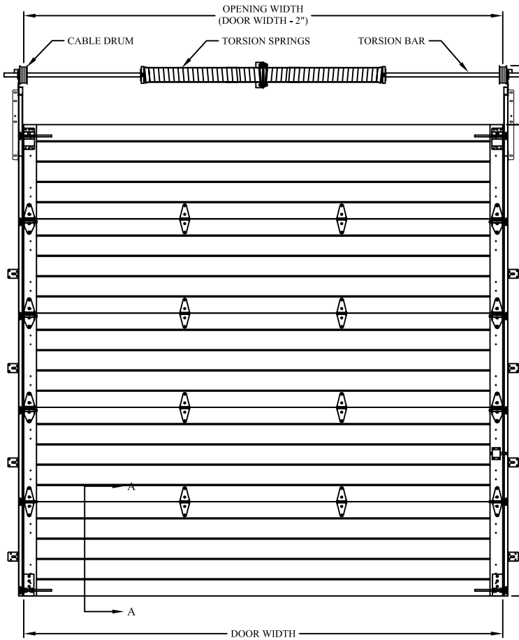
INTERIOR ELEVATION
