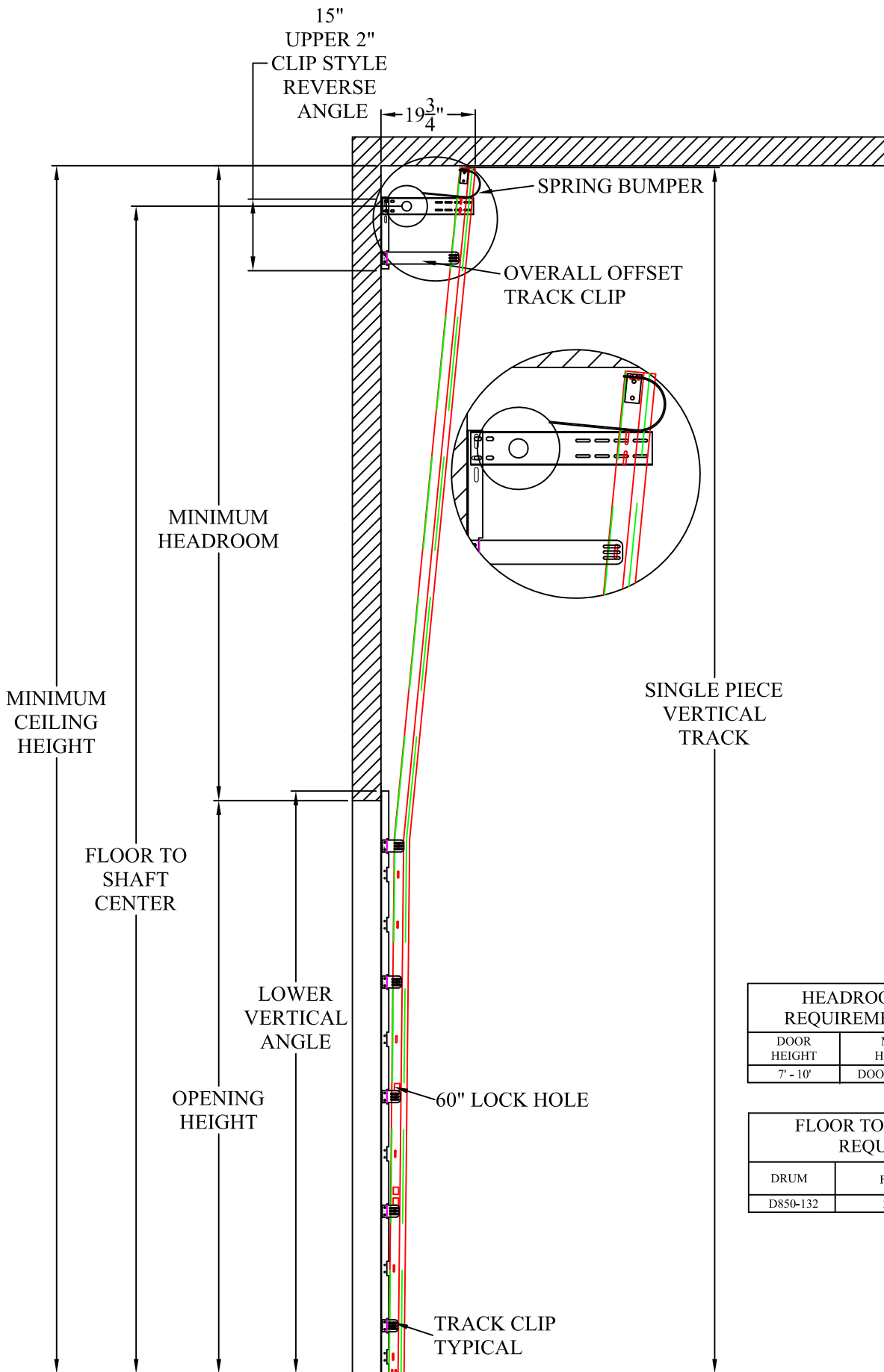
RAPID INSTALL VERTICAL LIFT 3" TRACK SET DETAIL
